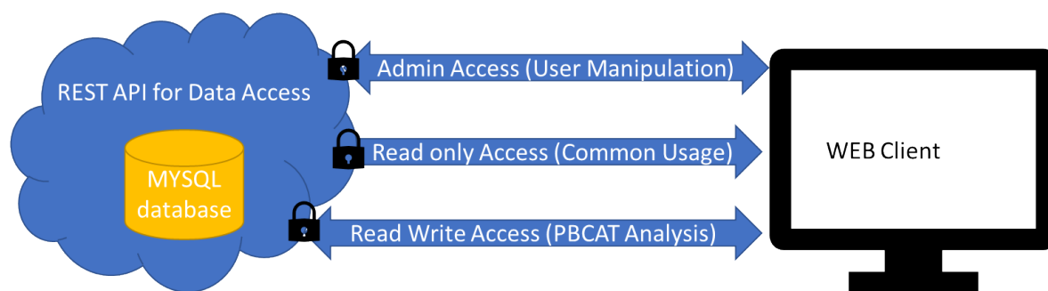
Figure 6.1 Schematic of the Software Design. The three critical components of the application developed for this project are the database, the REST API for data access, and the Web (browser) Client to display results
