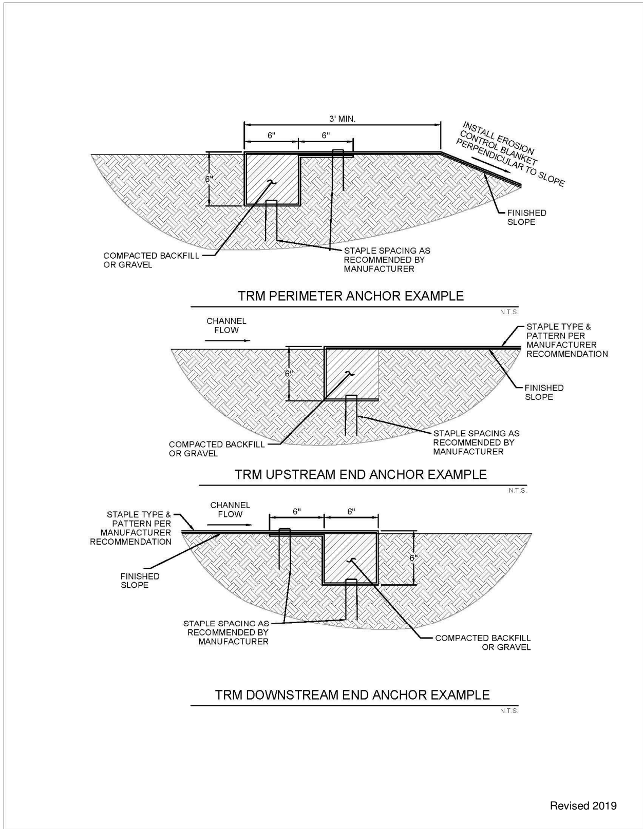
Figure 2.15 Examples of Turf Reinforcement Mat Anchoring (Source: Modified from Texas Department of Transportation Soil Retention Blanket Product Installation Sheet)
