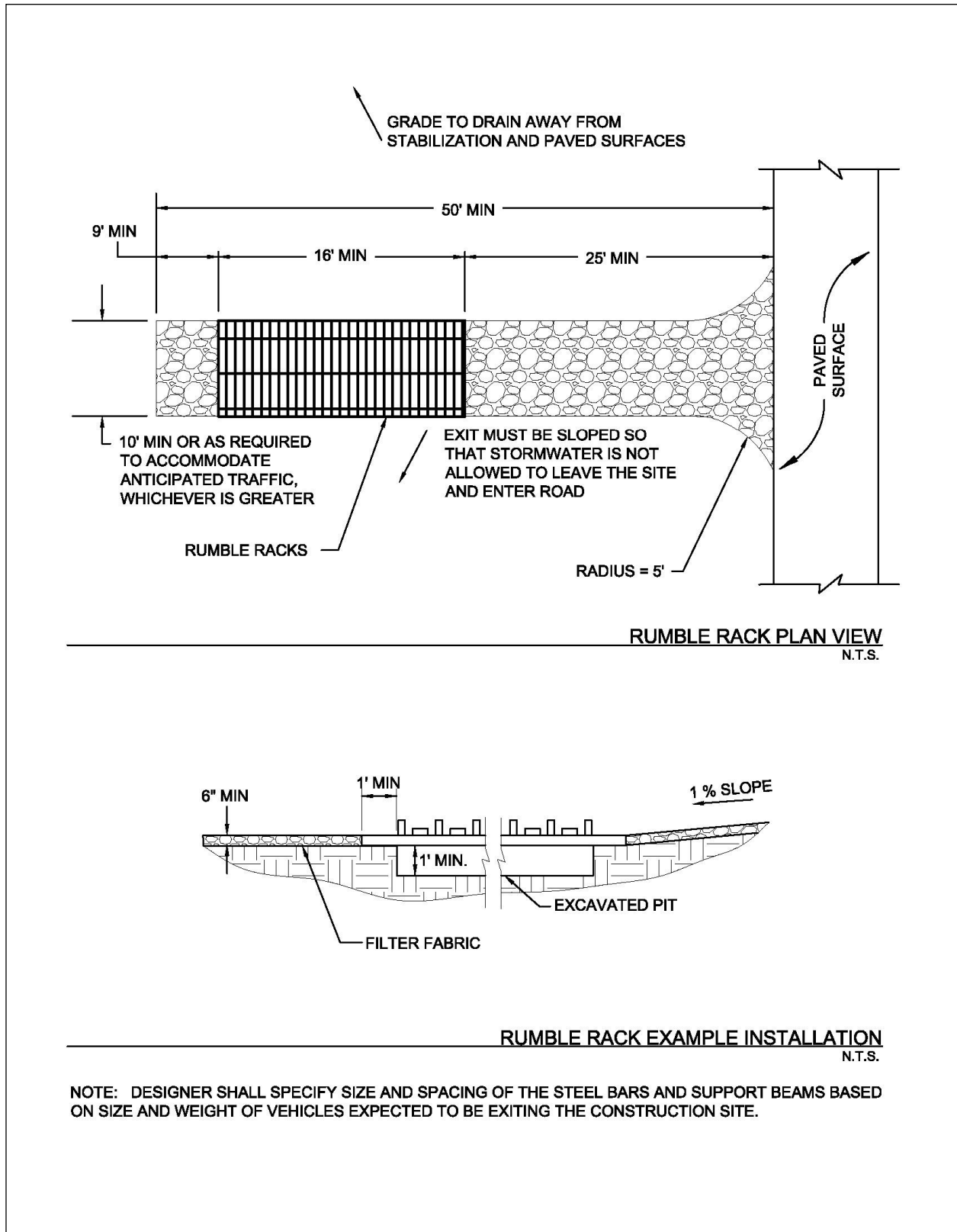
Figure 3.41 Schematics of Rumble Rack Wheel Cleaning
