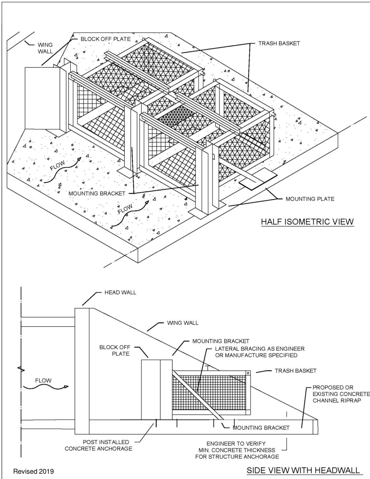
Figure 4.2 Trash Rack Isometric
