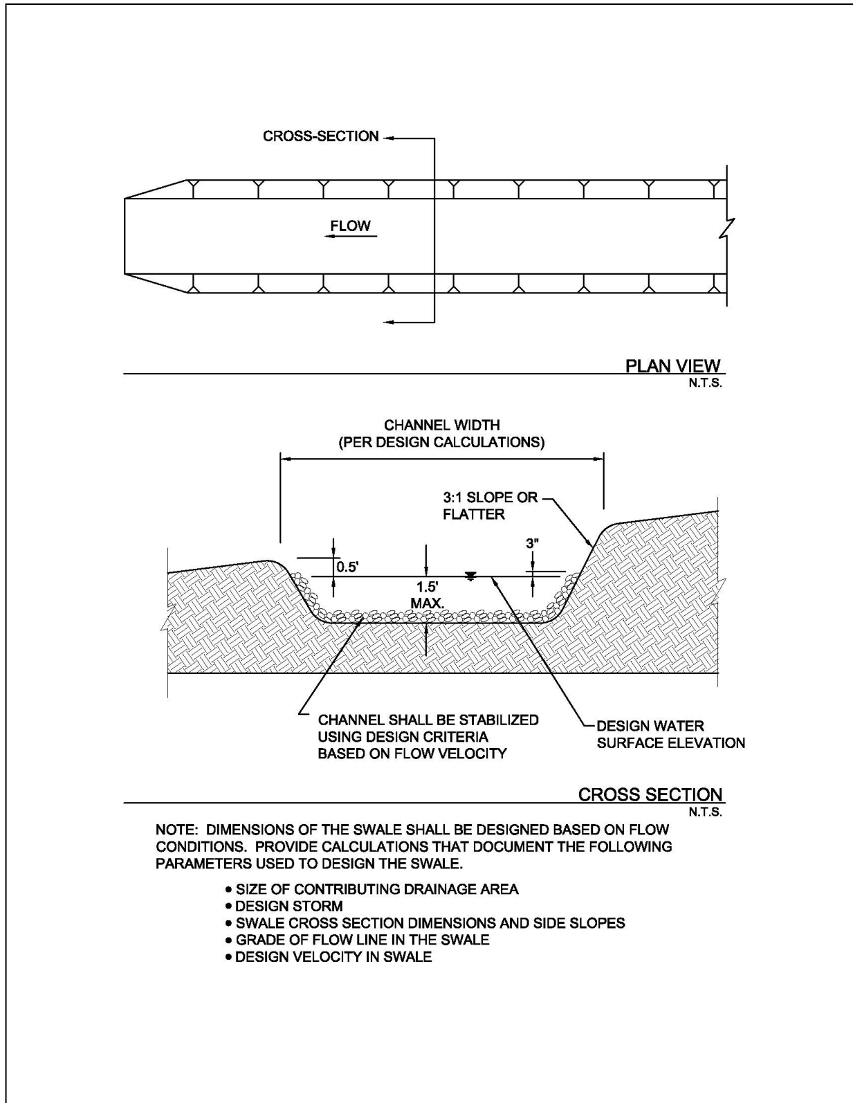
Figure 2.11 Schematics of Interceptor Swale
