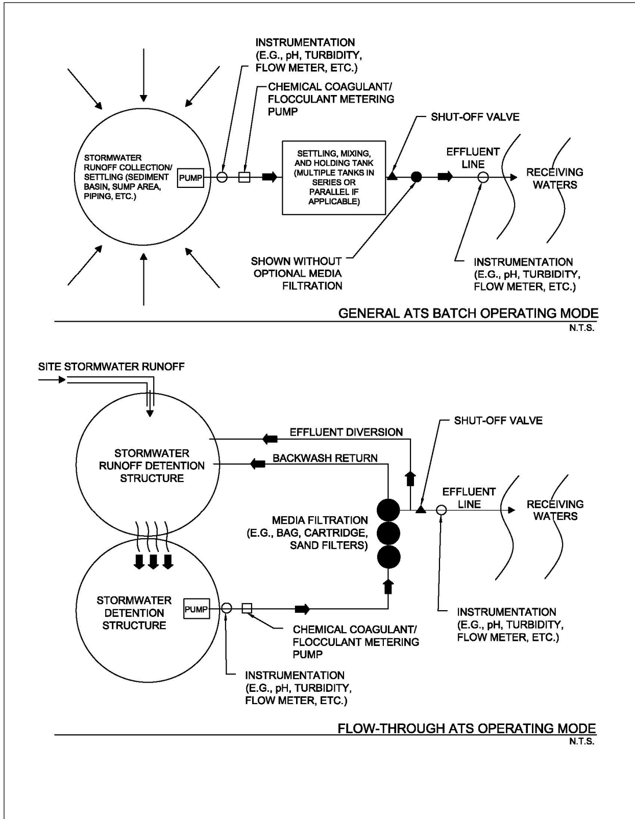
Figure 3.1 Schematics of Active Treatment Systems
