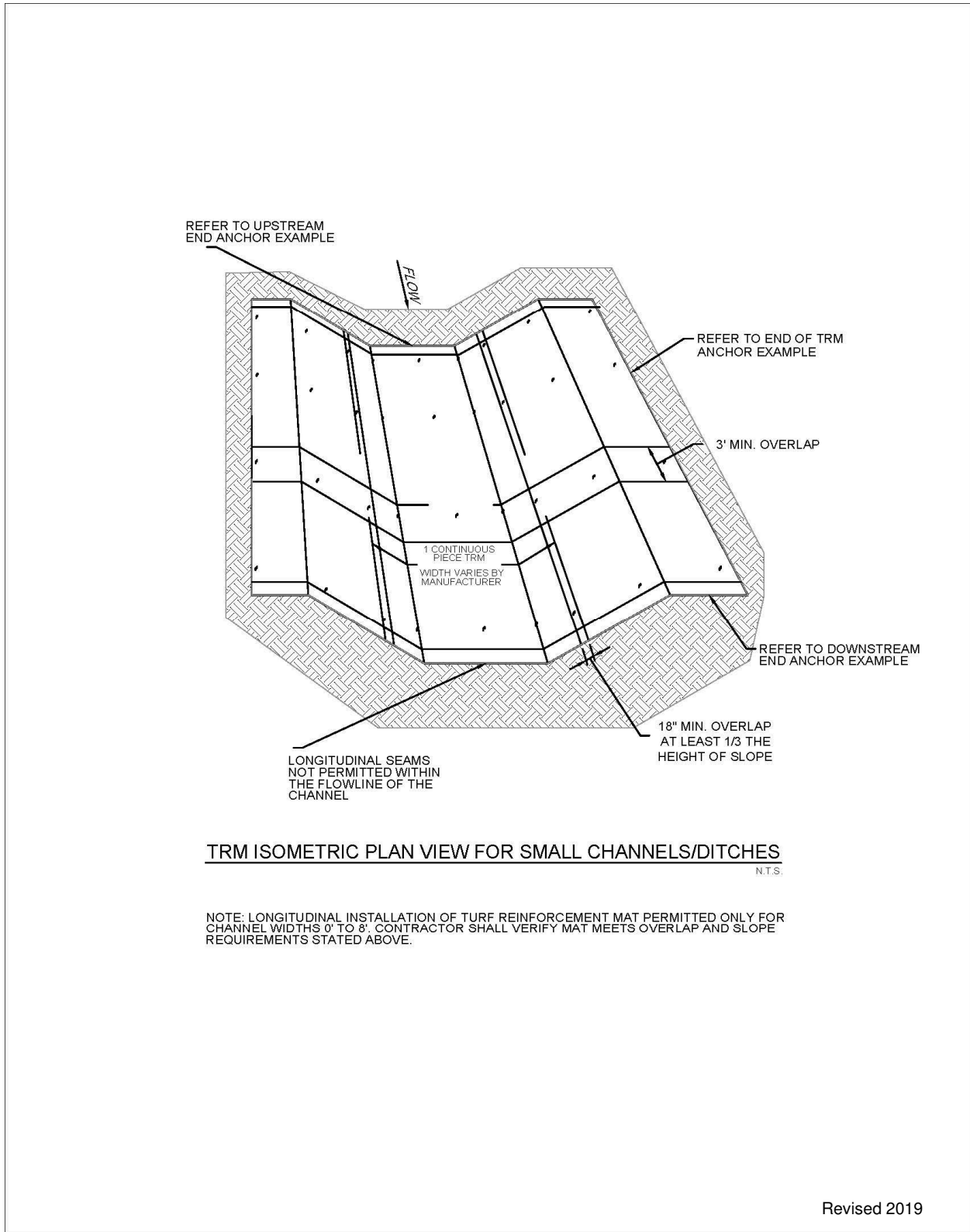
Figure 2.14 Permanent Turf Reinforcement Mats
