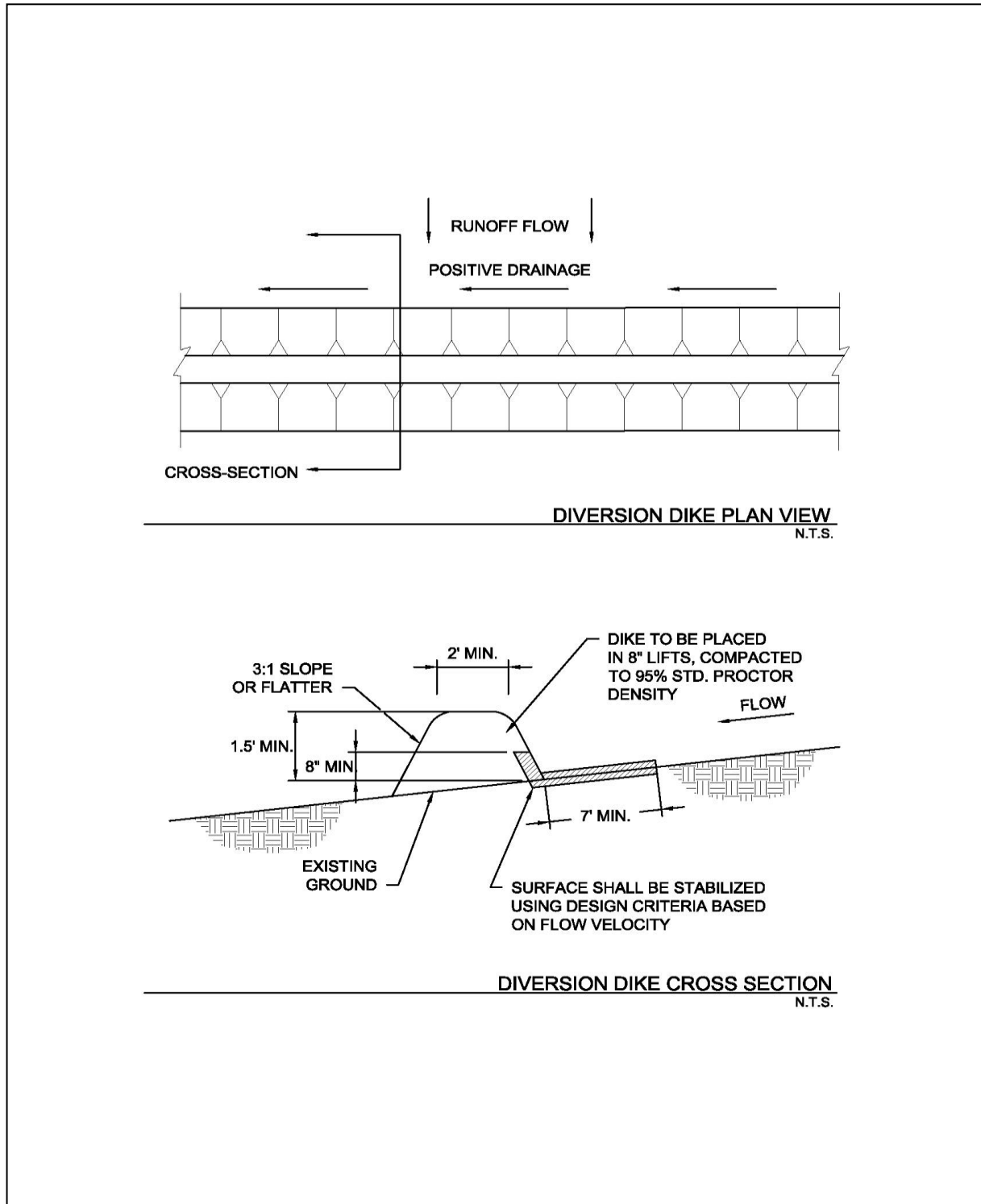
Figure 2.6 Schematics of Diversion Dike
