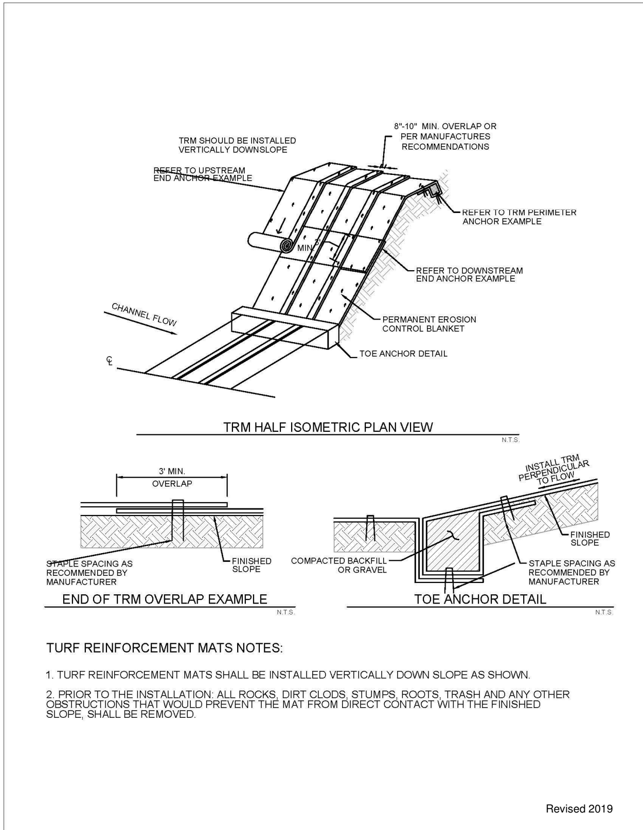
Figure 2.13 Schematics of Turf Reinforcement Mats
