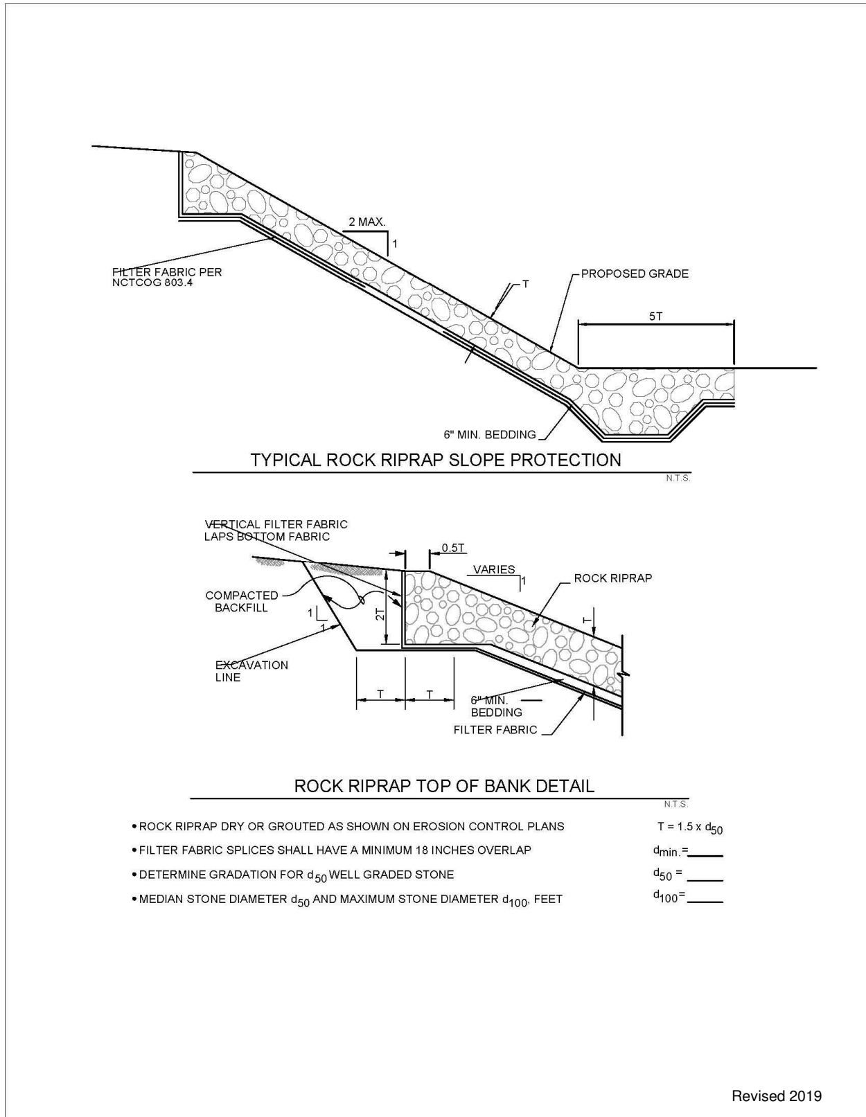
Figure 2.16 Riprap Schematics of Rock Riprap
