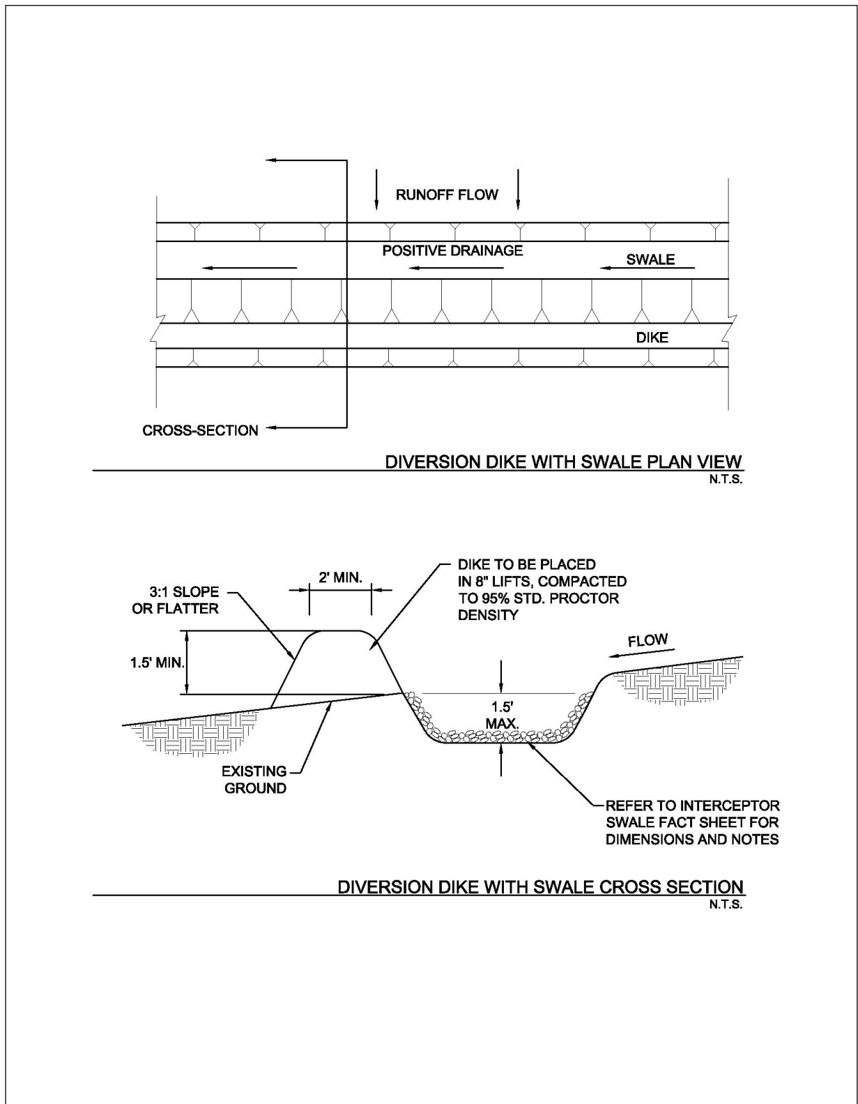
Figure 2.7 Schematics of Diversion Dike with Swale
