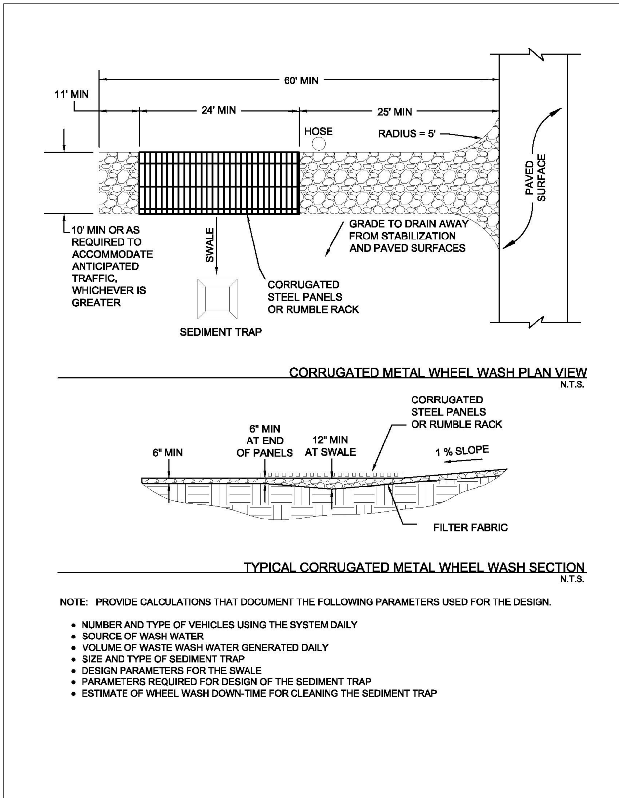
Figure 3.42 Schematics of Corrugated Metal Wheel Wash
