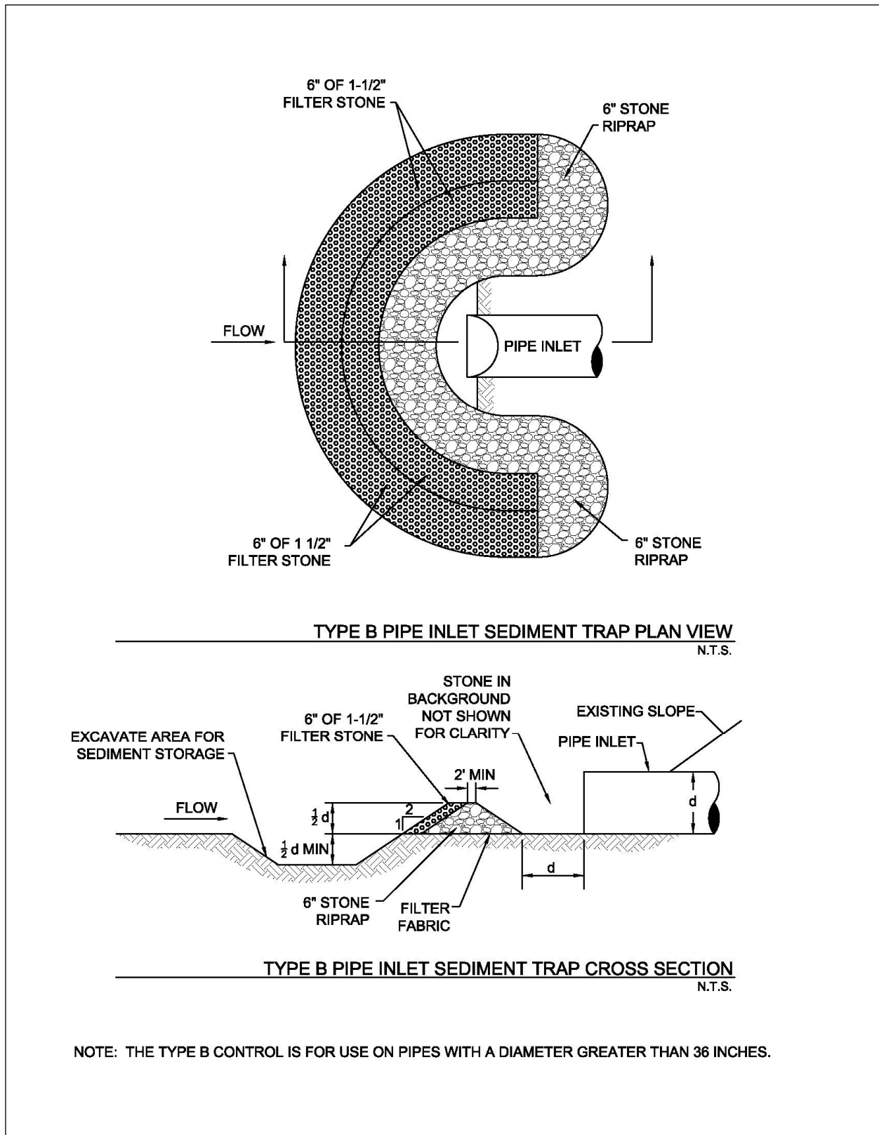
Figure 3.20 Schematics of Type B Pipe Inlet Sediment Trap
