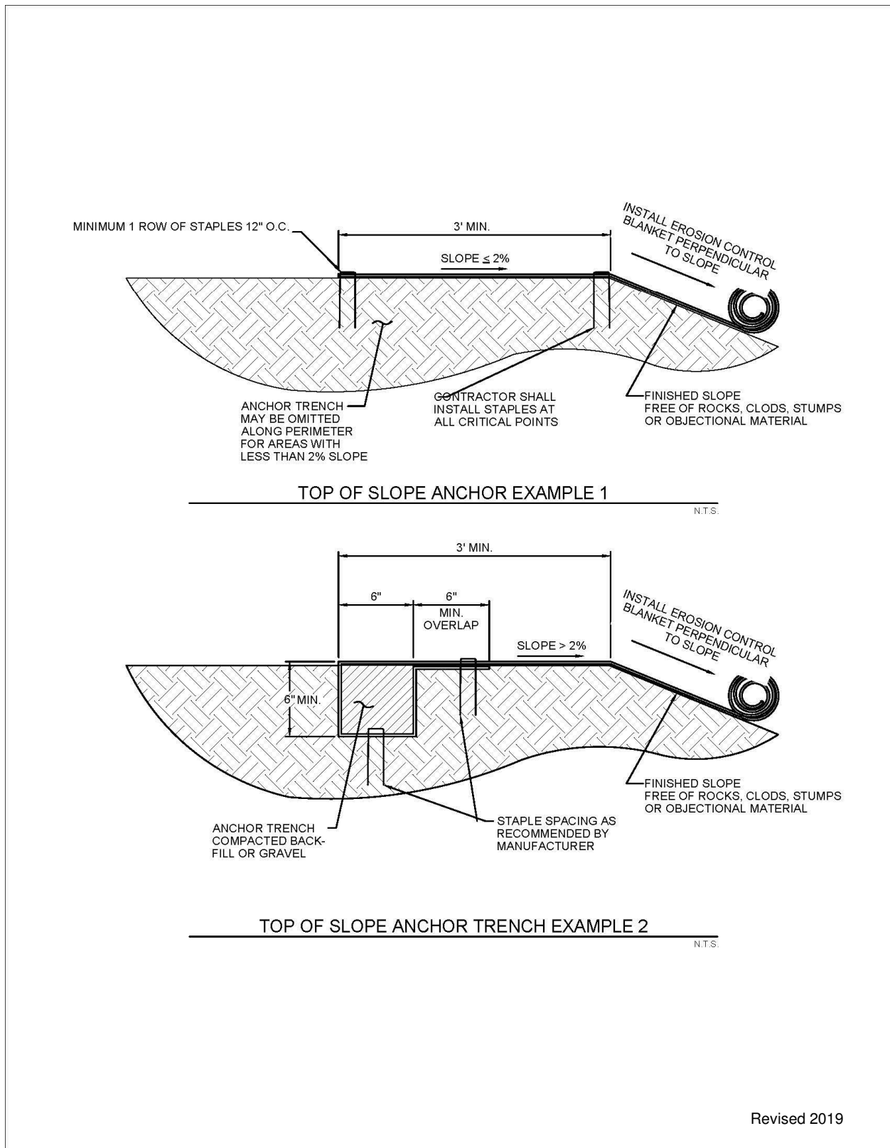
Figure 2.9 Anchor Examples for Erosion Control Blankets
