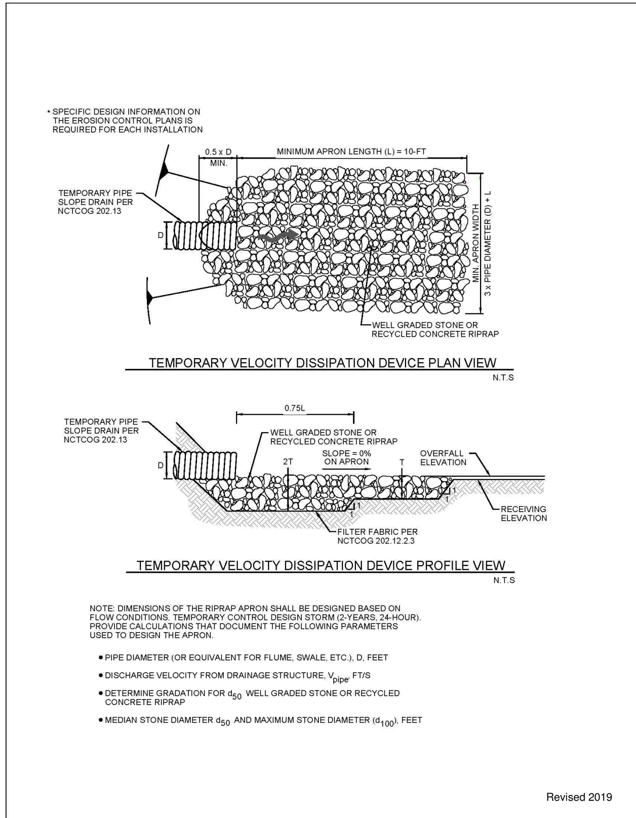
Figure 2.18 Schematics of Velocity Dissipation Device (Source: Modified from Oklahoma City Public Works Engineering Division Detail ERO-A17)
