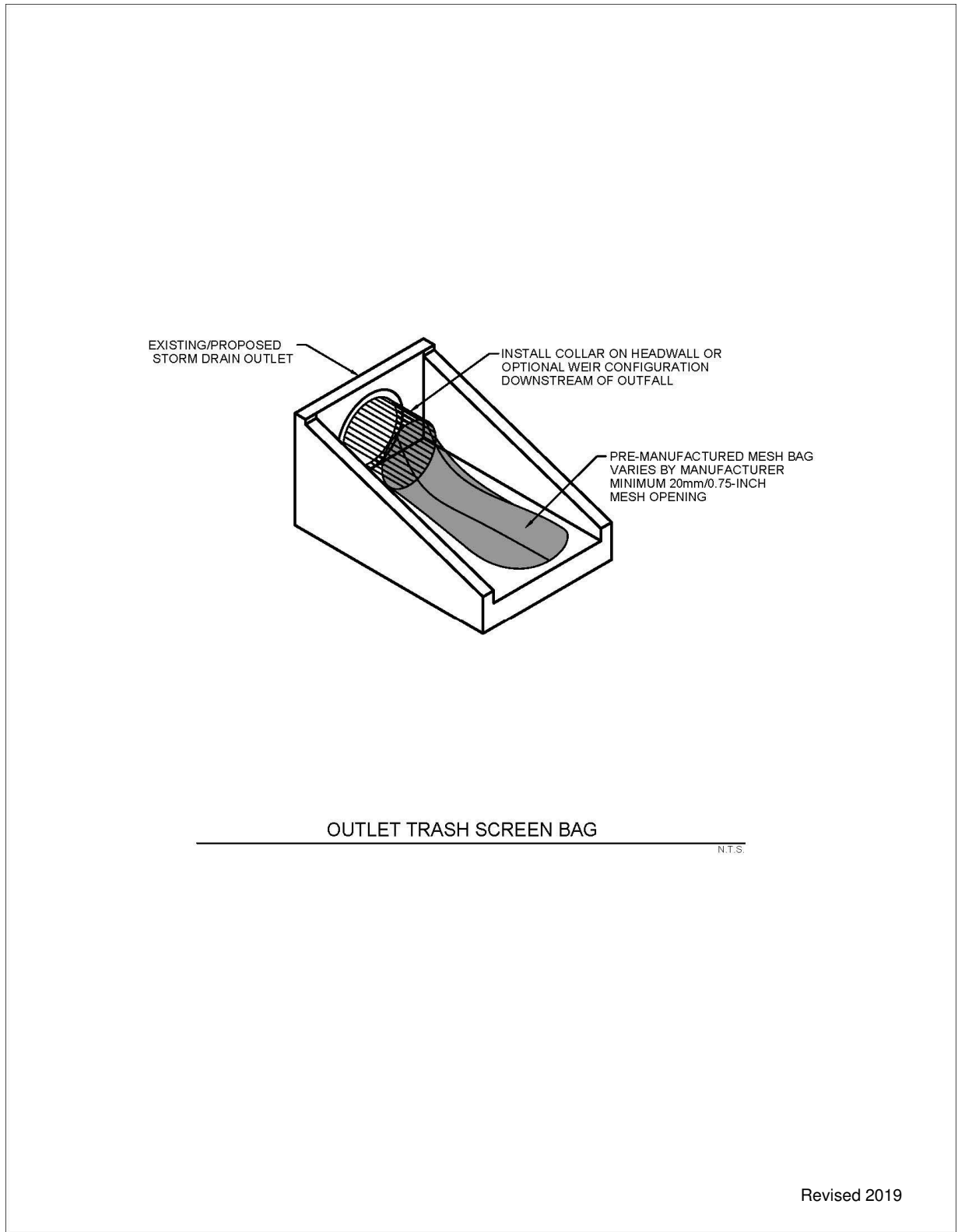
Figure 4.5 Schematic Outlet Trash Screen Bag
