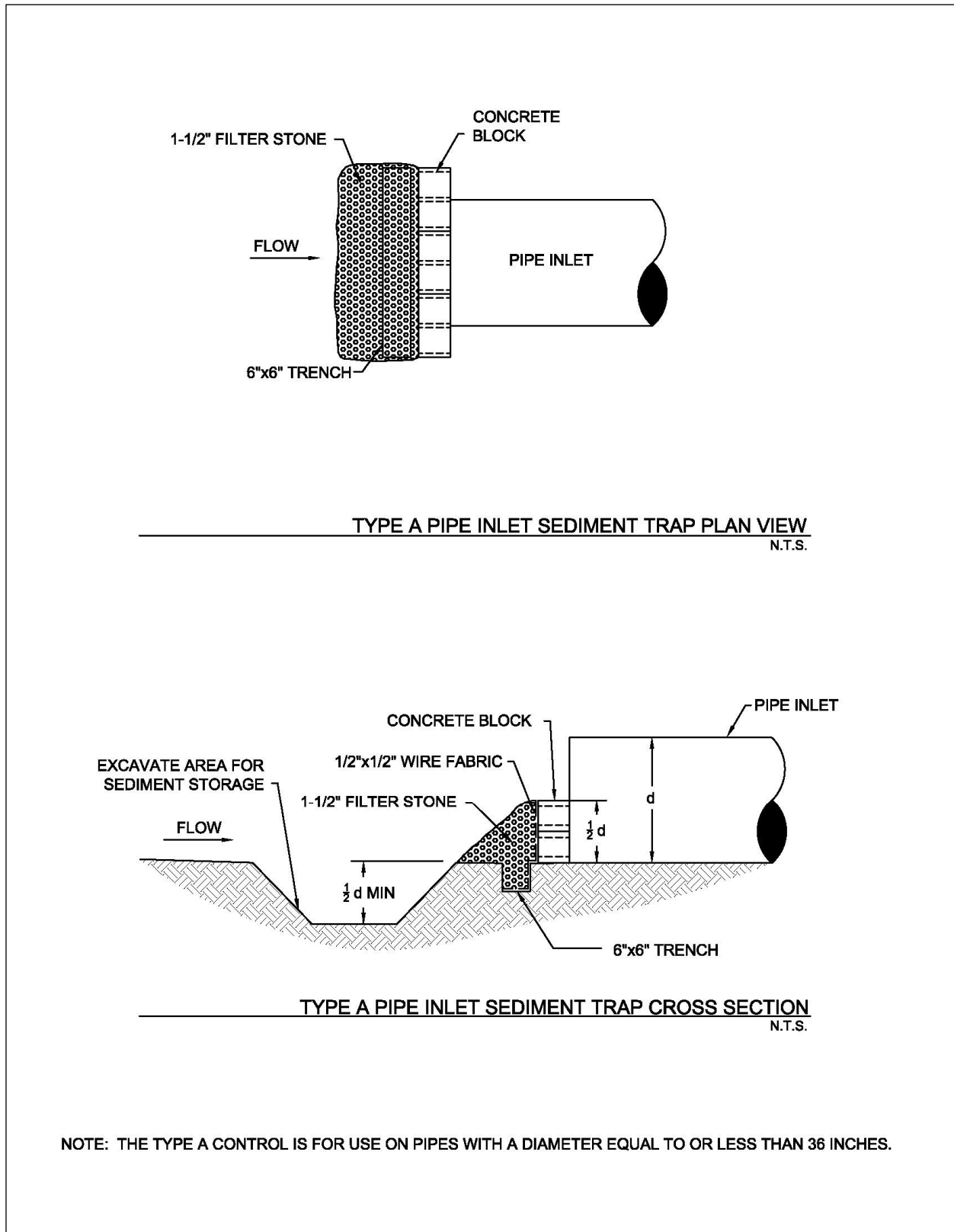
Figure 3.19 Schematics of Type A Pipe Inlet Sediment Trap
