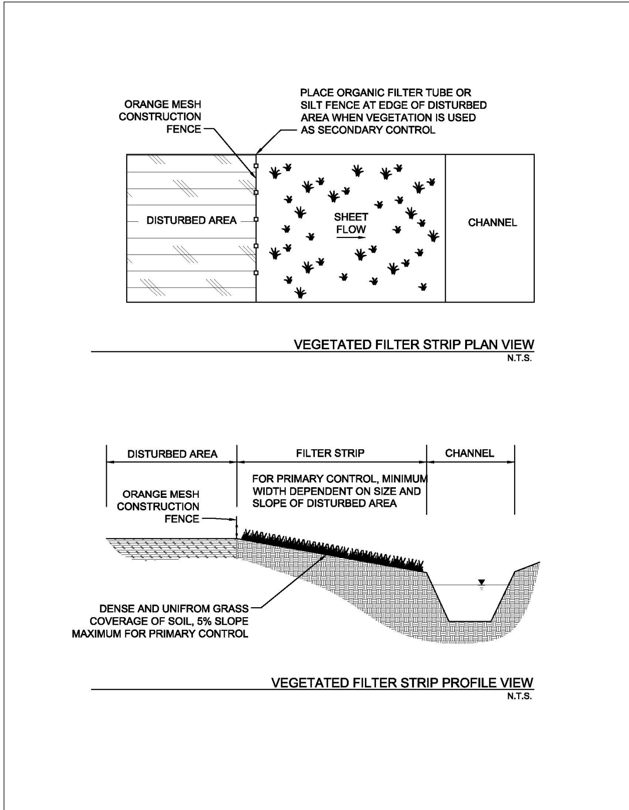
Figure 3.40 Schematics of Vegetated Filter Strip
