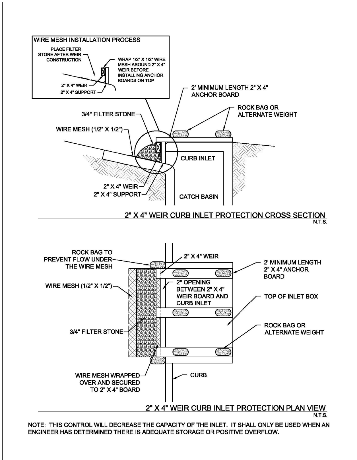
Figure 3.5 Schematics of 2"x4" Weir Curb Inlet Protection
