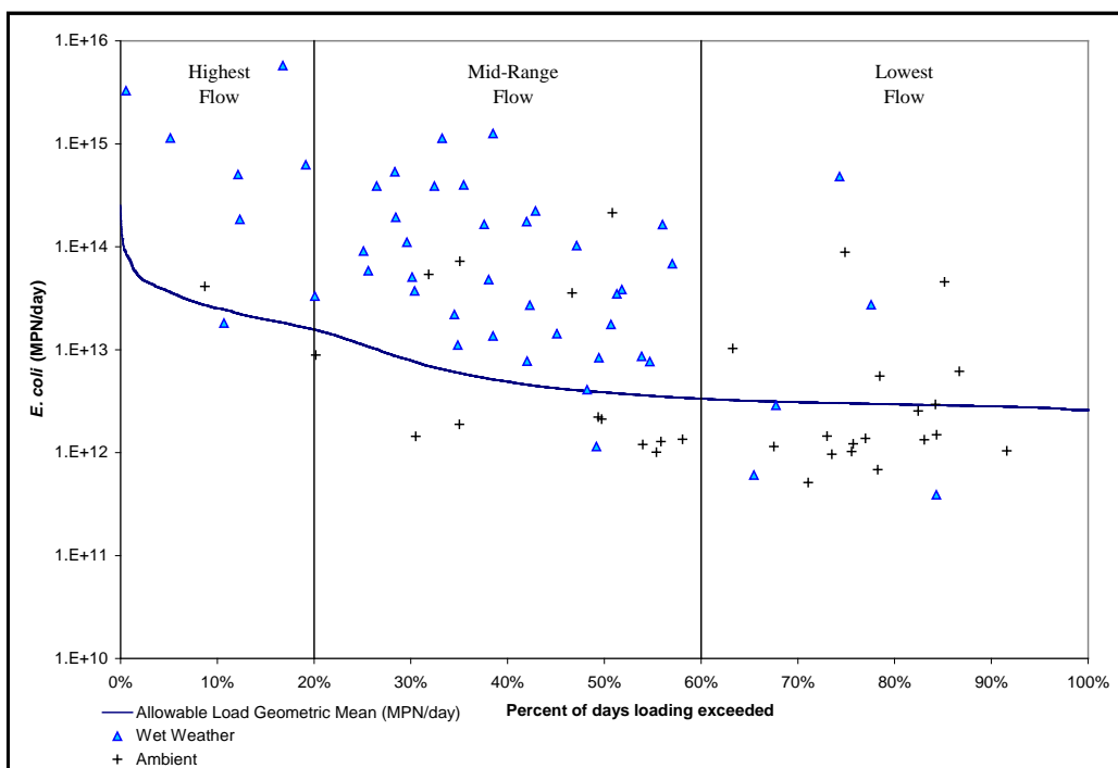
Figure 6. Load duration curve for station 10934 (AU 0805_03). E. coli samples collected within 4 days of a precipitation event are designated as triangles.
