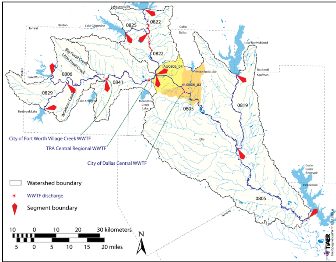
Figure A-2. Upper Trinity River and major tributaries showing large wastewater treatment facilities and study area
