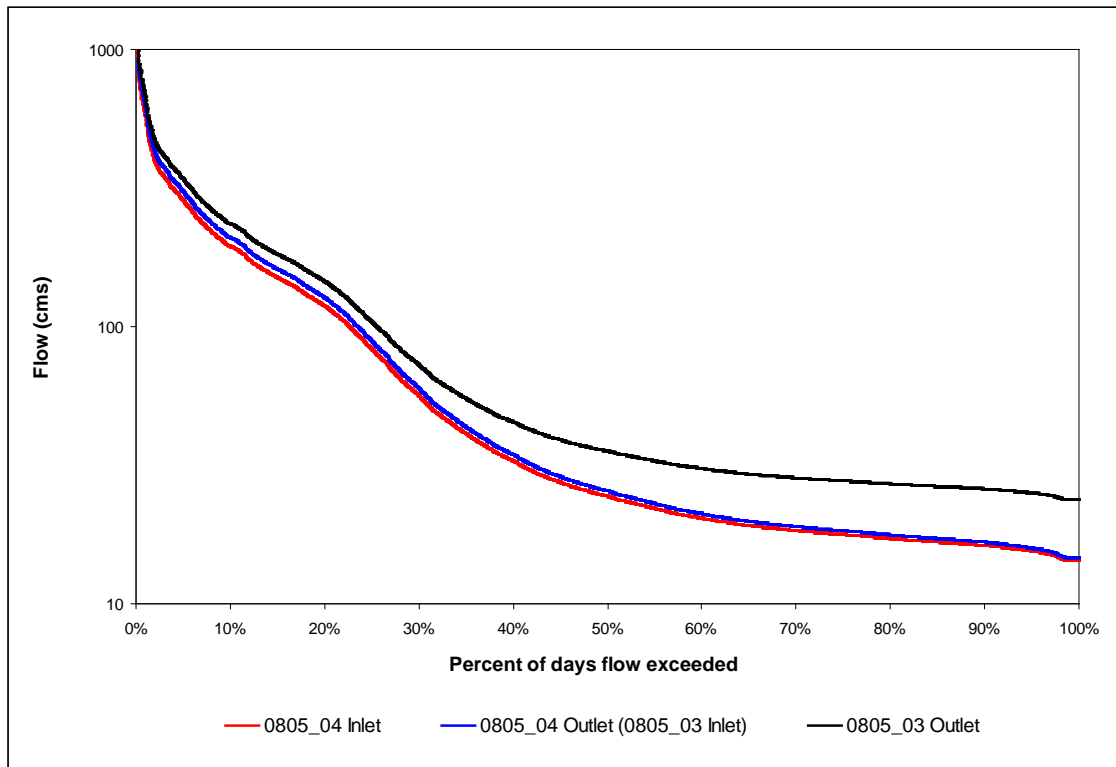
Figure A-3. Flow duration curves for 0805_04 and 0805_03
