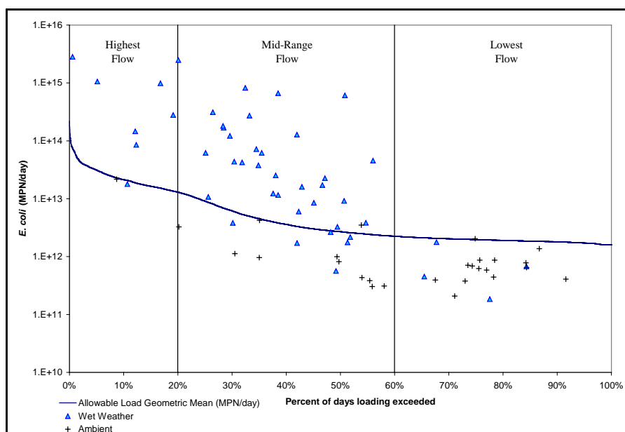
Figure 5. Load duration curve for station 10937 (AU 0805_04). E. coli samples collected within 4 days of a precipitation event are designated as triangles.
