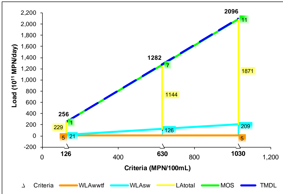
Figure B-2. Allocation loads for 0805_03 as a function of water quality criteria
