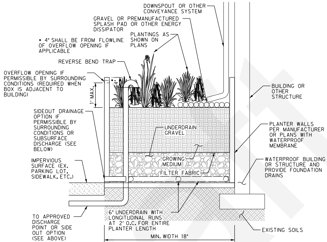
FLOW-THROUGH PLANTER NOT TO SCALE
