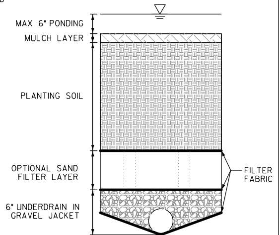
MEDIA CUT SECTION NOT TO SCALE
